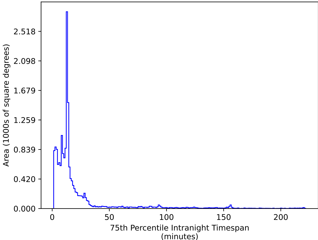
roll_pause_mjdp180_v3.4_10yrs WFD i band: 75th Percentile Intranight Timespan
