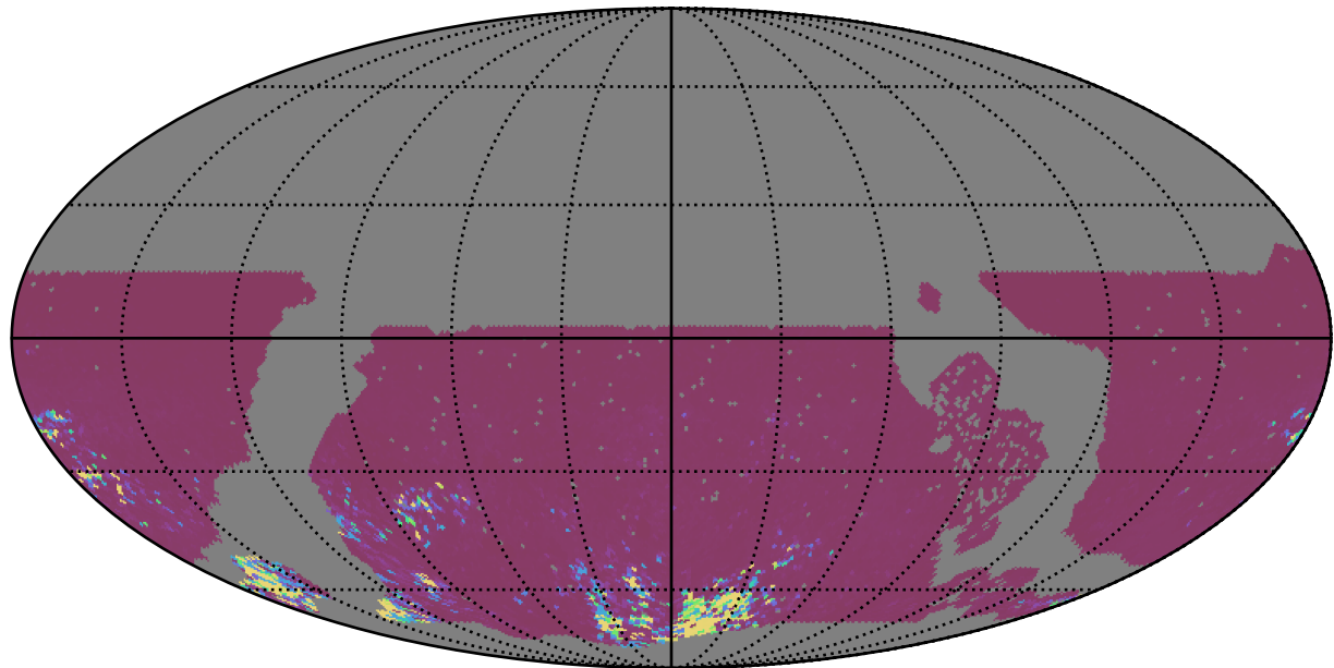
roll_pause_mjdp180_v3.4_10yrs WFD gr bands: 75th Percentile Intranight Timespan
