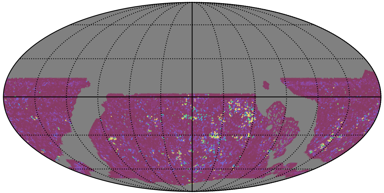
roll_pause_mjdp180_v3.4_10yrs WFD g band: 75th Percentile Intranight Timespan
