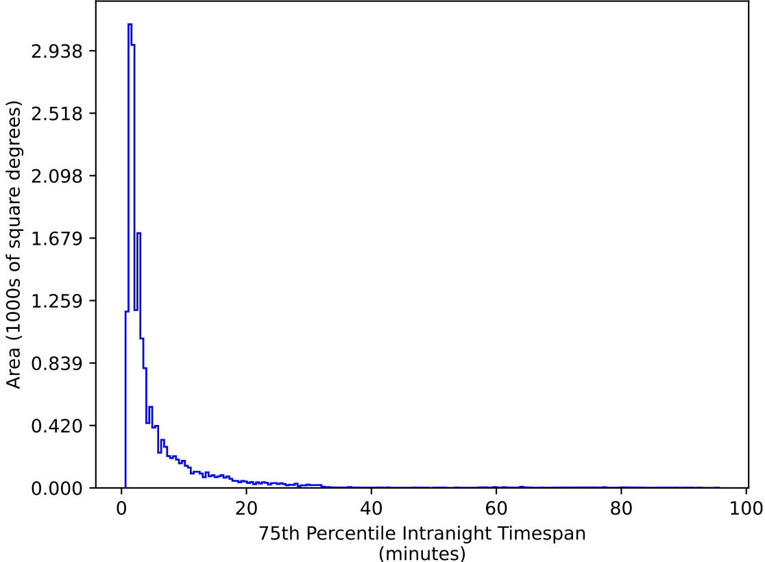
roll_pause_mjdp180_v3.4_10yrs WFD g band: 75th Percentile Intranight Timespan
