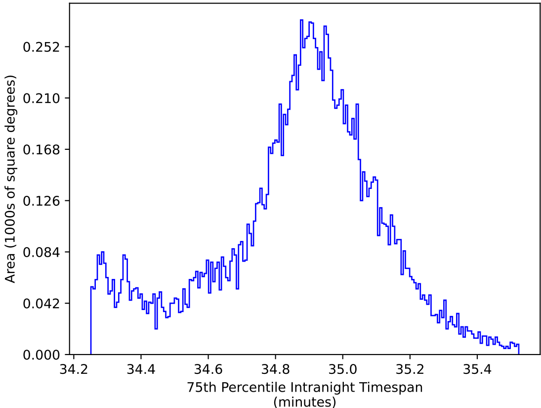
roll_pause_mjdp180_v3.4_10yrs WFD all bands: 75th Percentile Intranight Timespan
