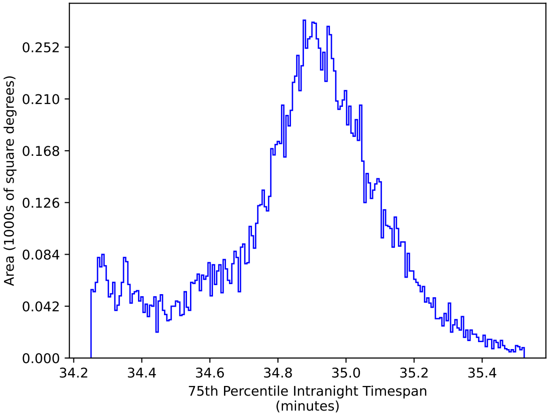
roll_pause_mjdp180_v3.4_10yrs WFD: 75th Percentile Intranight Timespan
