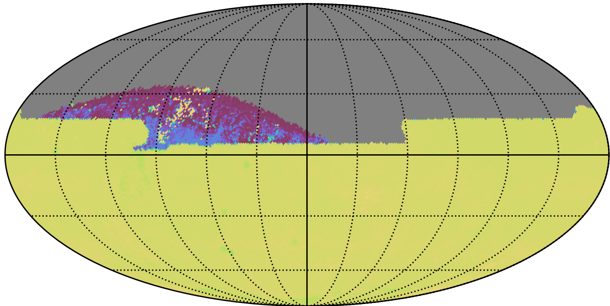
roll_pause_mjdp180_v3.4_10yrs All sky zy bands: 75th Percentile Intranight Timespan
