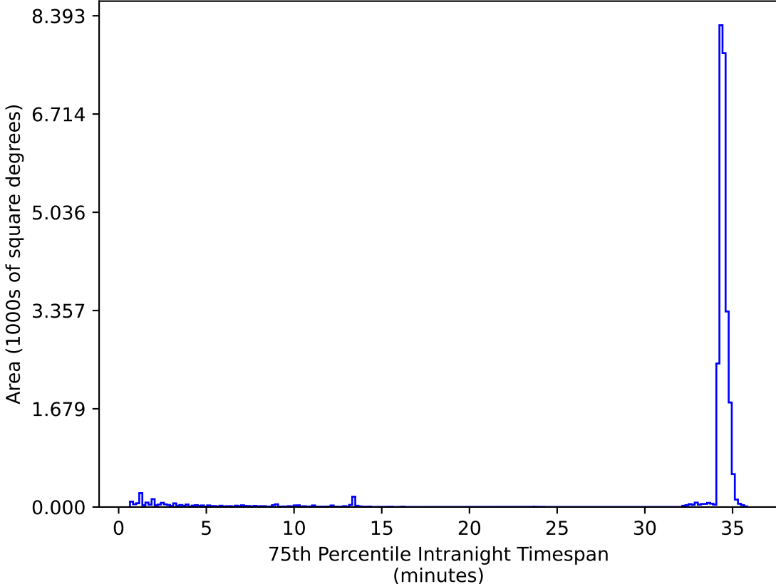
roll_pause_mjdp180_v3.4_10yrs All sky zy bands: 75th Percentile Intranight Timespan
