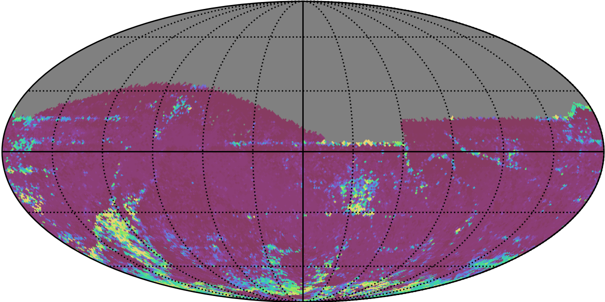
roll_pause_mjdp180_v3.4_10yrs All sky z band: 75th Percentile Intranight Timespan
