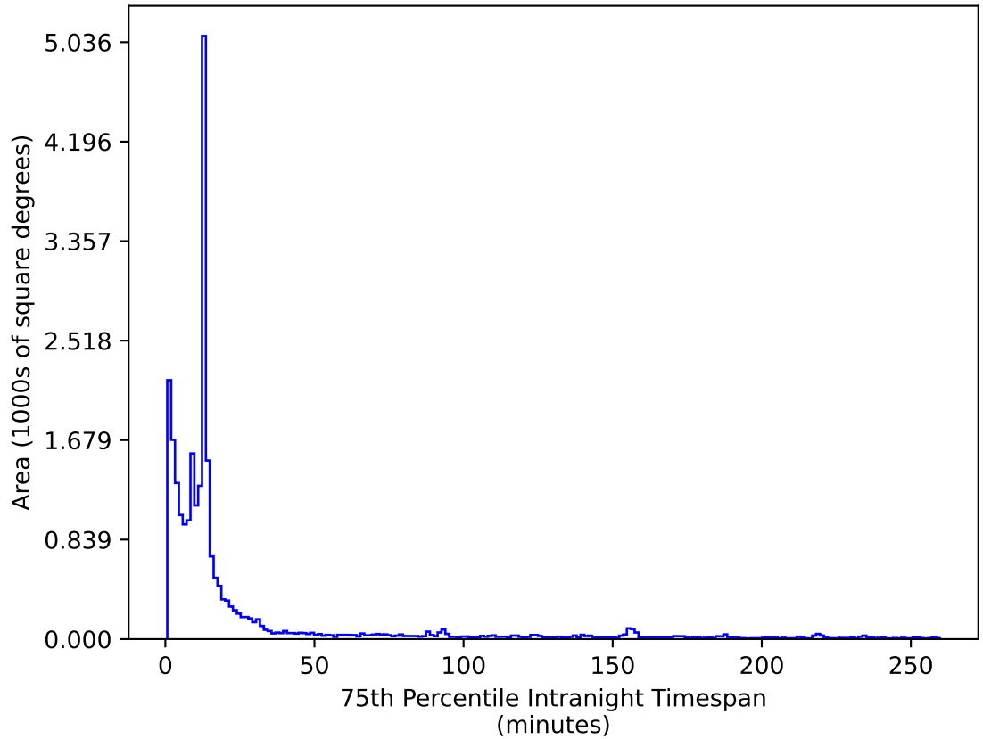
roll_pause_mjdp180_v3.4_10yrs All sky z band: 75th Percentile Intranight Timespan
