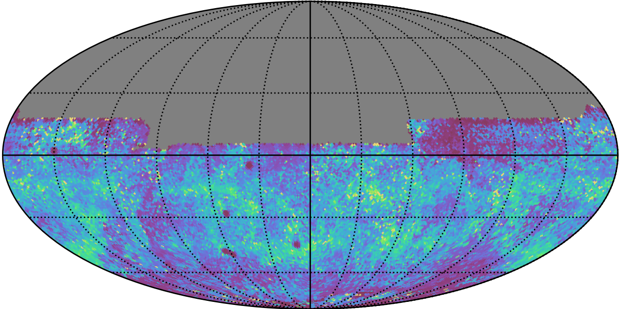
roll_pause_mjdp180_v3.4_10yrs All sky y band: 75th Percentile Intranight Timespan
