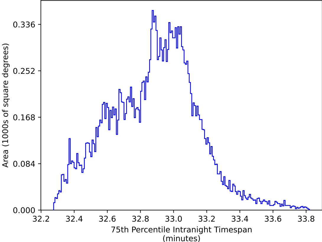
roll_pause_mjdp180_v3.4_10yrs All sky y band: 75th Percentile Intranight Timespan
