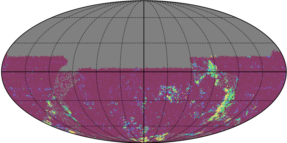
roll_pause_mjdp180_v3.4_10yrs All sky u band: 75th Percentile Intranight Timespan
