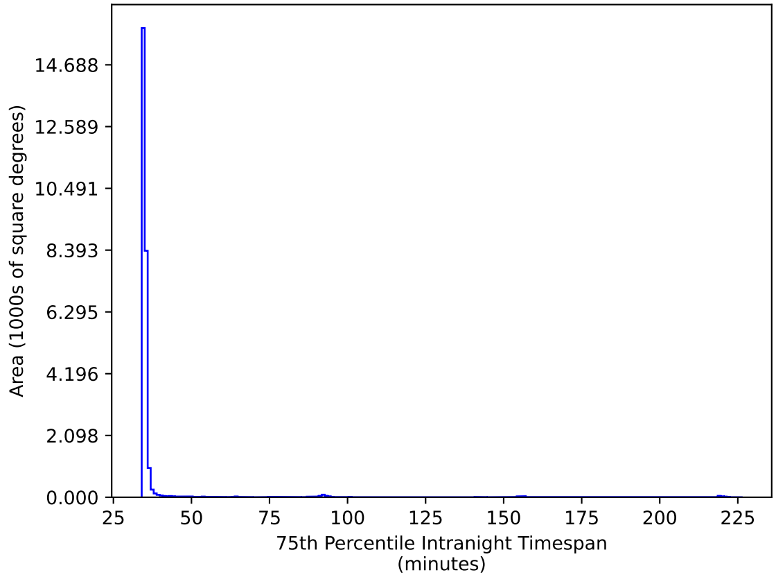
roll_pause_mjdp180_v3.4_10yrs All sky ri bands: 75th Percentile Intranight Timespan
