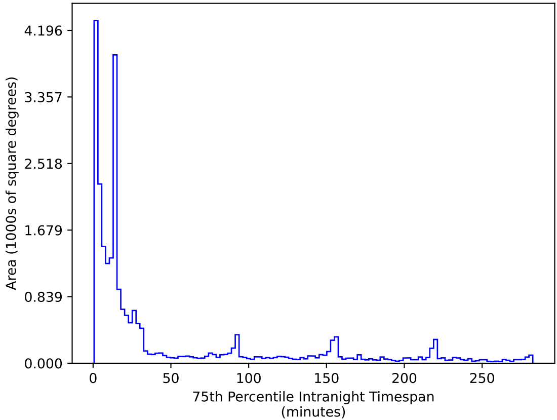
roll_pause_mjdp180_v3.4_10yrs All sky r band: 75th Percentile Intranight Timespan
