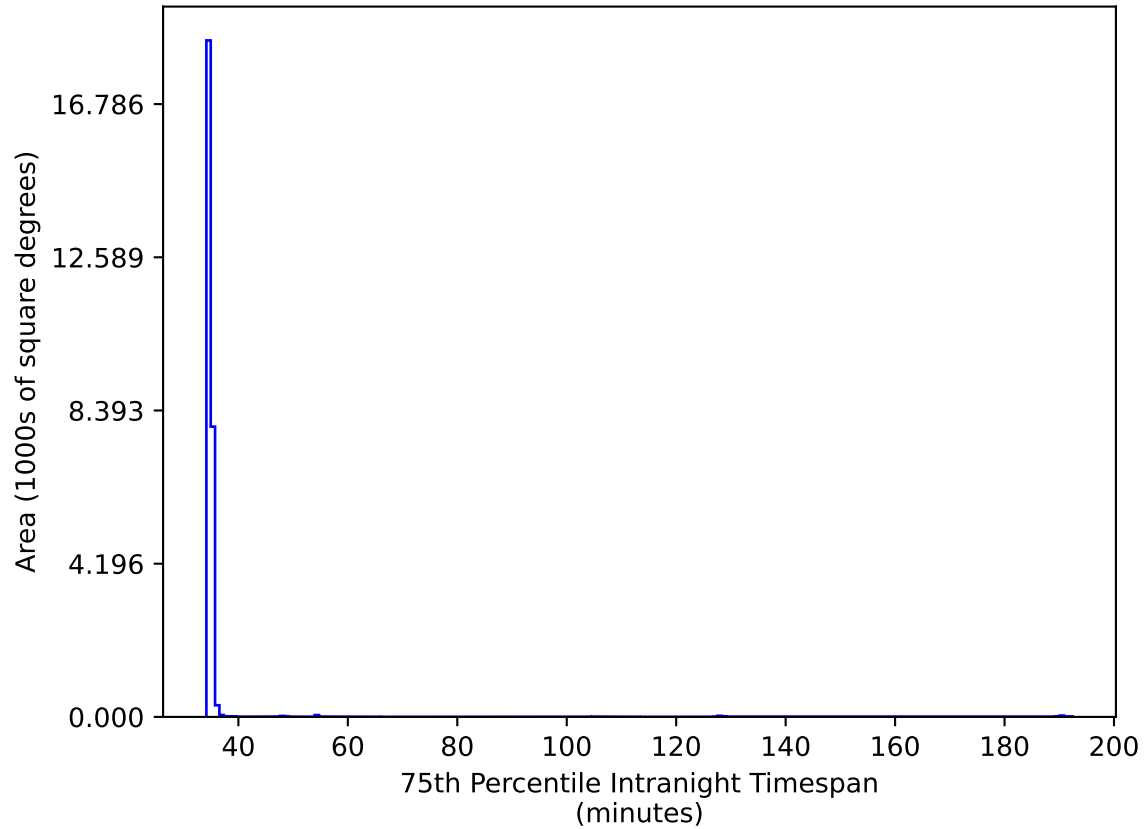
roll_pause_mjdp180_v3.4_10yrs All sky iz bands: 75th Percentile Intranight Timespan
