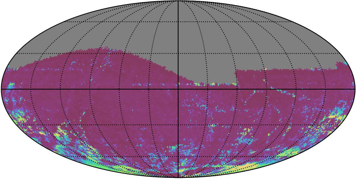
roll_pause_mjdp180_v3.4_10yrs All sky i band: 75th Percentile Intranight Timespan
