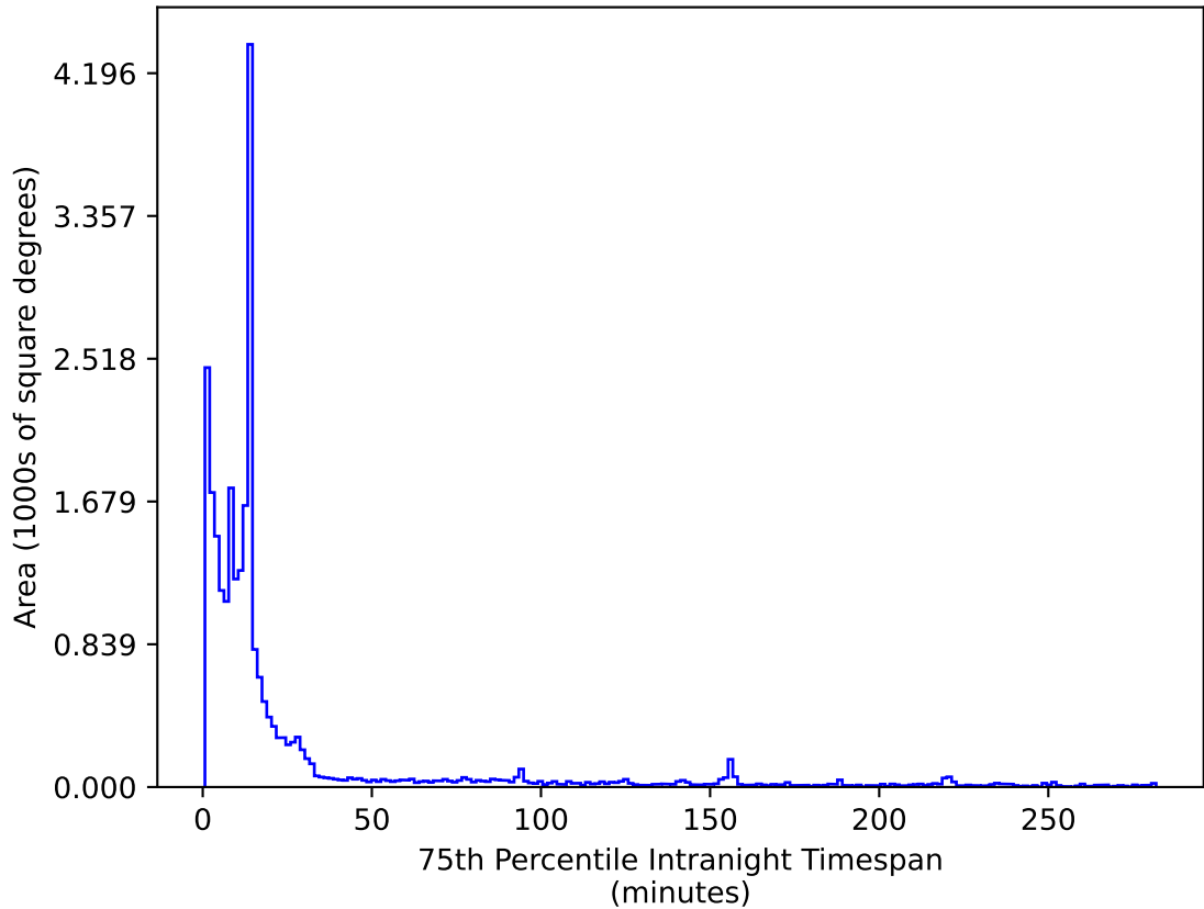
roll_pause_mjdp180_v3.4_10yrs All sky i band: 75th Percentile Intranight Timespan
