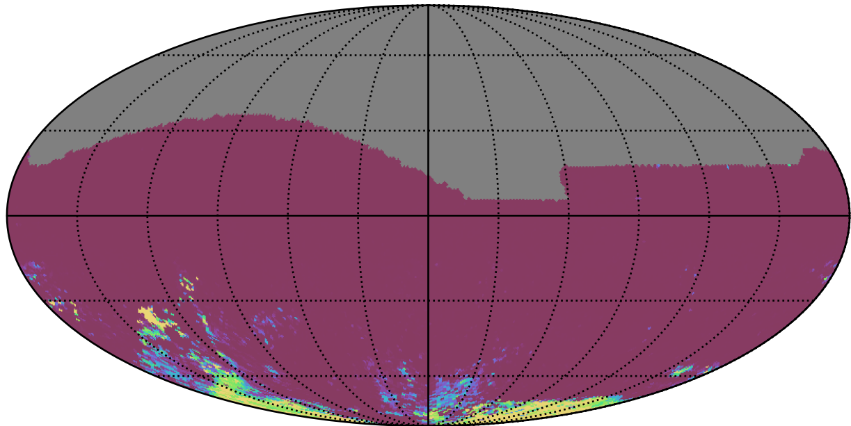
roll_pause_mjdp180_v3.4_10yrs All sky gr bands: 75th Percentile Intranight Timespan
