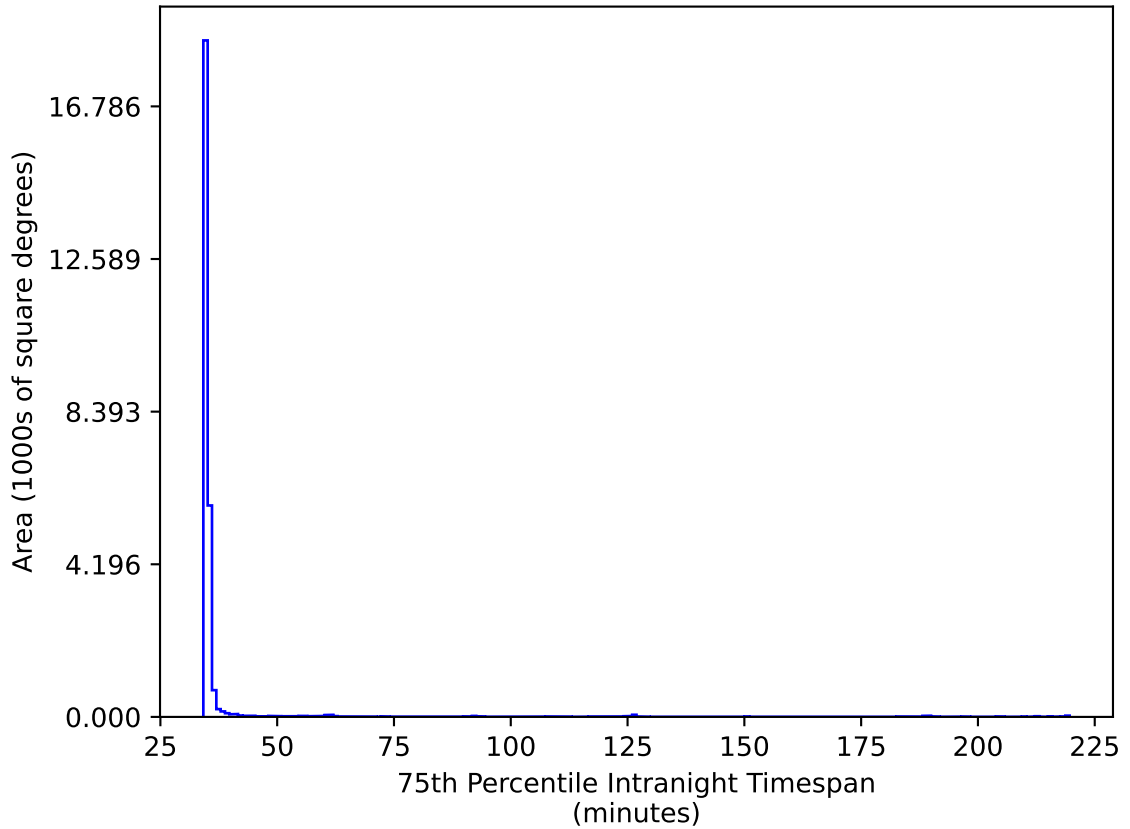
roll_pause_mjdp180_v3.4_10yrs All sky gr bands: 75th Percentile Intranight Timespan
