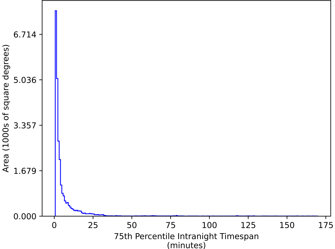
roll_pause_mjdp180_v3.4_10yrs All sky g band: 75th Percentile Intranight Timespan
