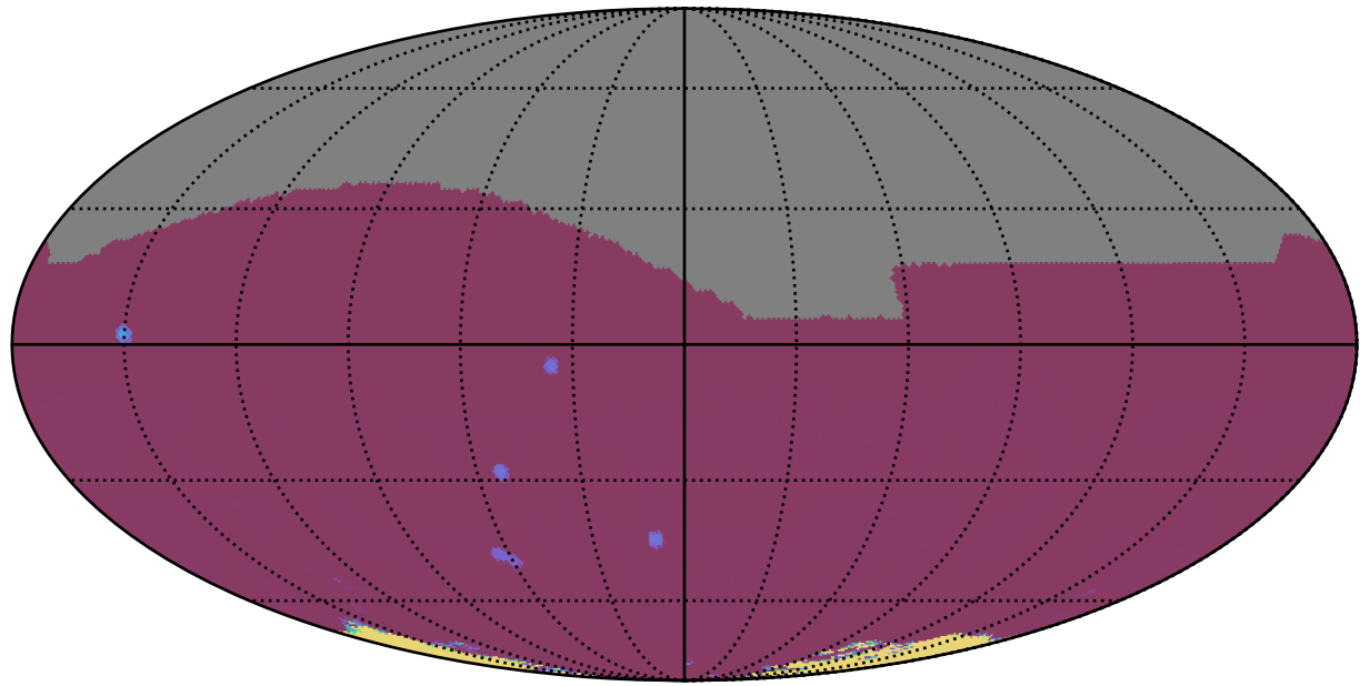
roll_pause_mjdp180_v3.4_10yrs All sky all bands: 75th Percentile Intranight Timespan
