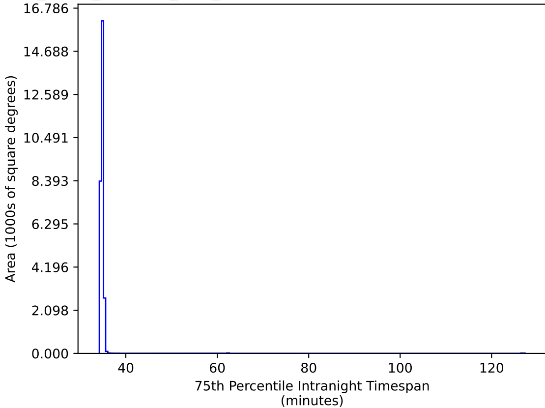
roll_pause_mjdp180_v3.4_10yrs All sky: 75th Percentile Intranight Timespan
