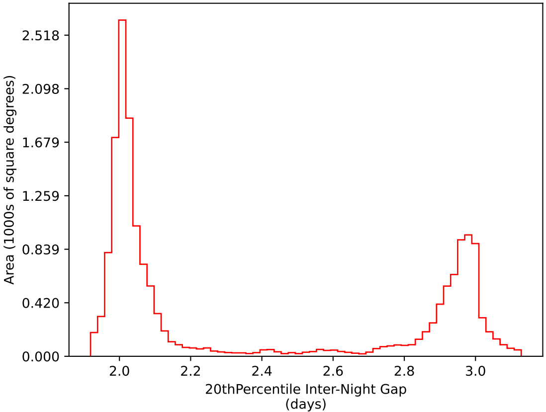
roll_pause_mjdp180_v3.4_10yrs WFD i band: 20thPercentile Inter-Night Gap
