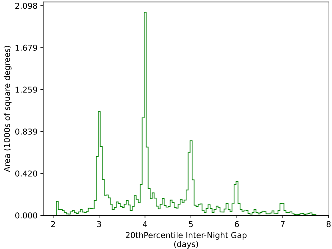
roll_pause_mjdp180_v3.4_10yrs WFD g band: 20thPercentile Inter-Night Gap
