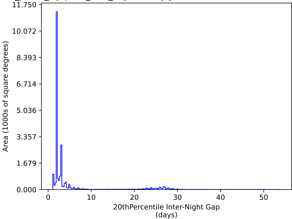
roll_pause_mjdp180_v3.4_10yrs All sky y band: 20thPercentile Inter-Night Gap
