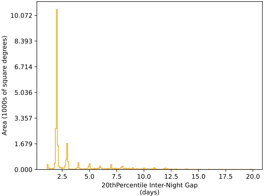
roll_pause_mjdp180_v3.4_10yrs All sky r band: 20thPercentile Inter-Night Gap
