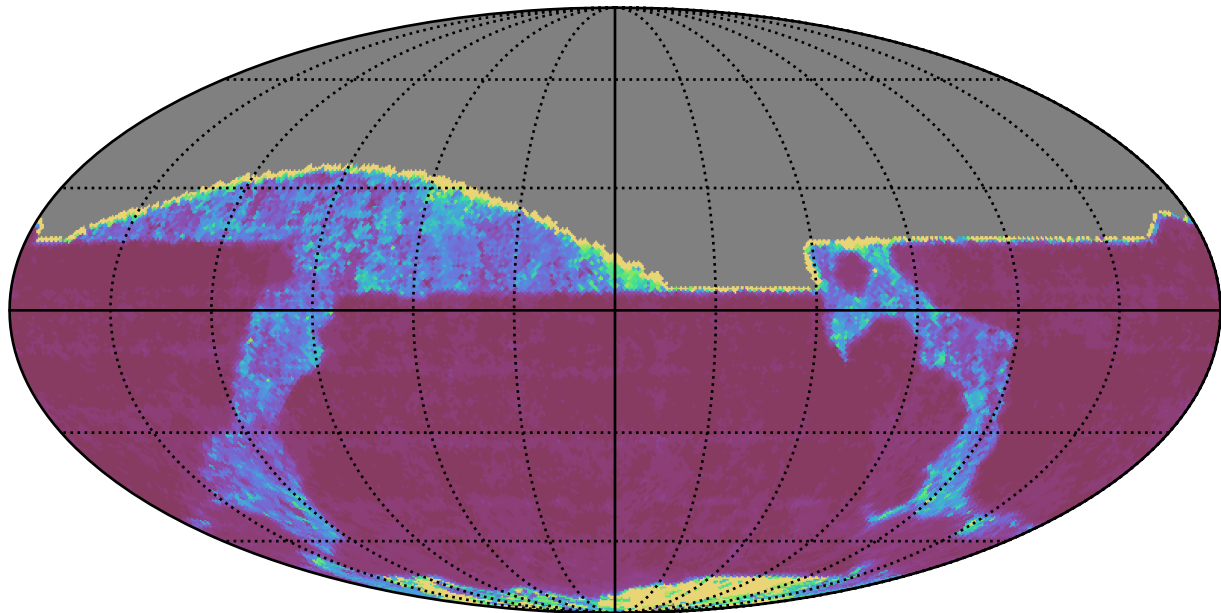
roll_pause_mjdp180_v3.4_10yrs All sky i band: 20thPercentile Inter-Night Gap
