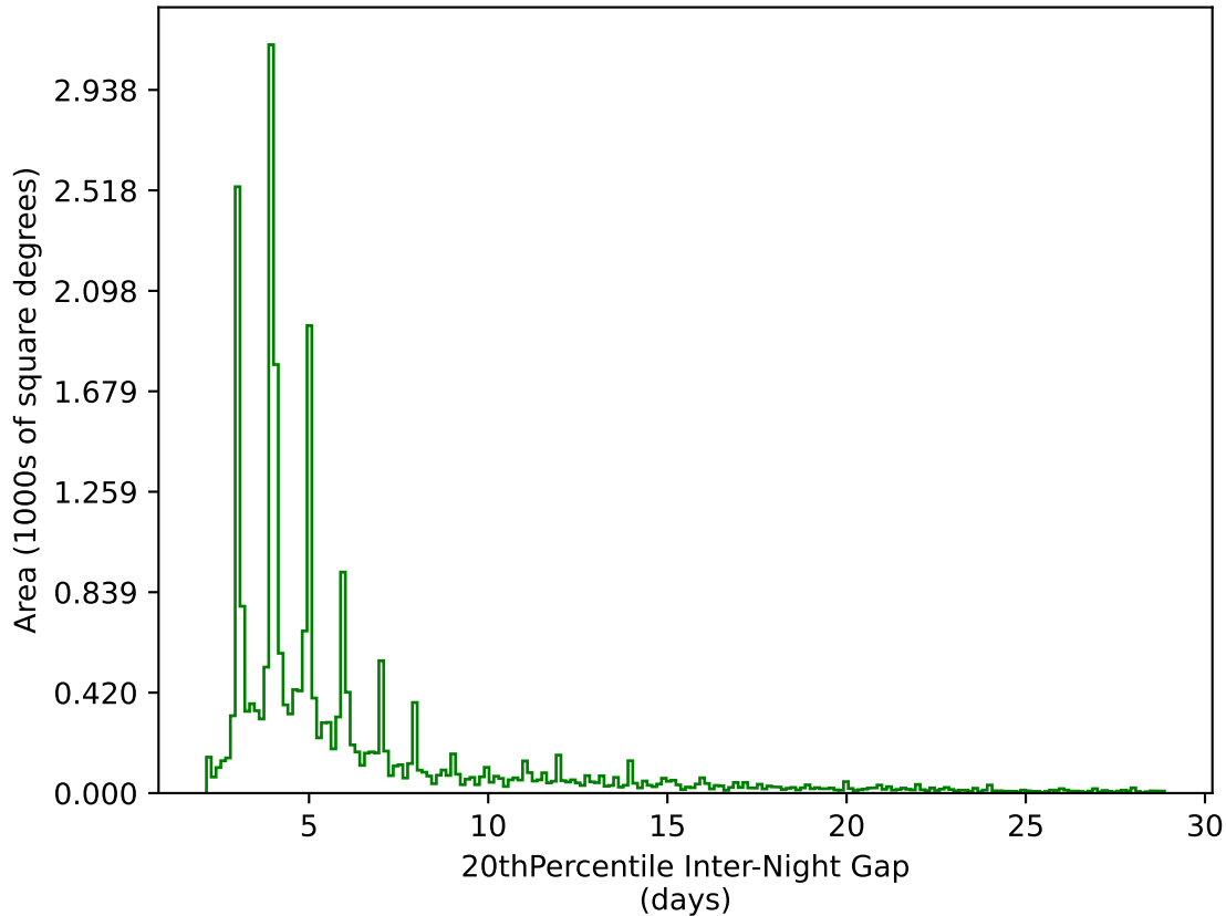
roll_pause_mjdp180_v3.4_10yrs All sky g band: 20thPercentile Inter-Night Gap
