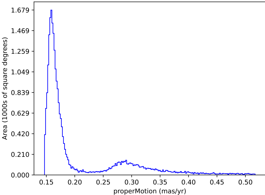
roll_pause_mjdp180_v3.4_10yrs : properMotion
