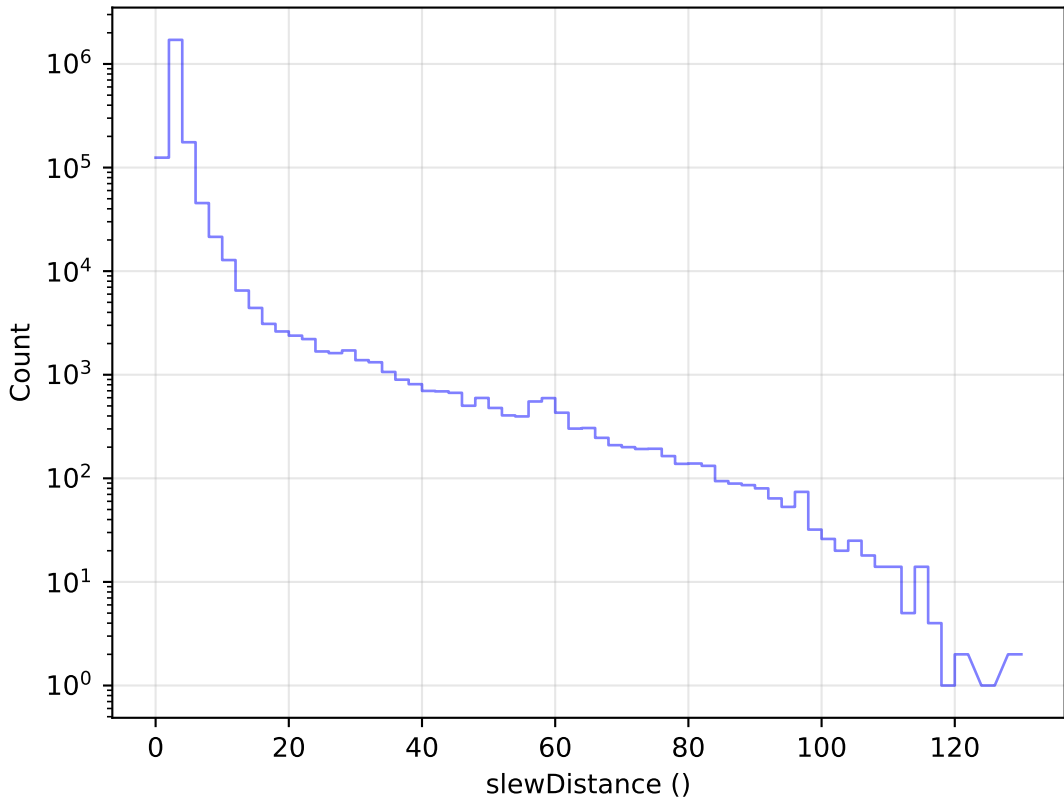
roll_pause_mjdp180_v3.4_10yrs All visits: Slew Distance Histogram
