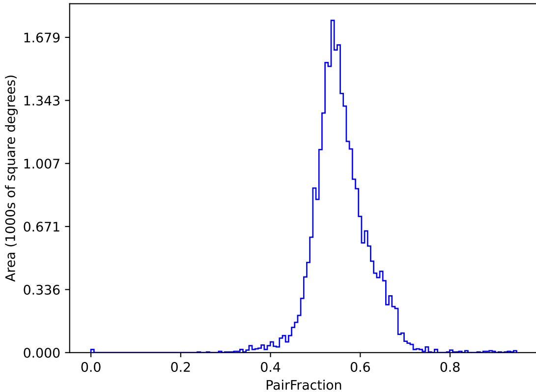
roll_pause_mjdp180_v3.4_10yrs (g or r or i): PairFraction
