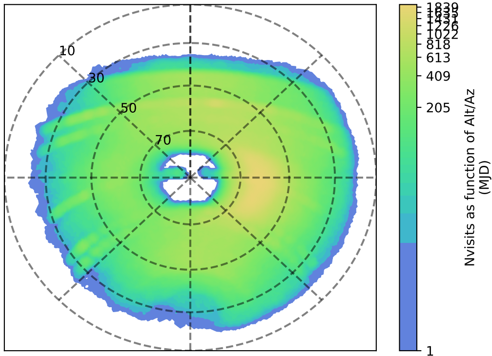
roll_pause_mjdp180_v3.4_10yrs y: Nvisits as function of Alt/Az
