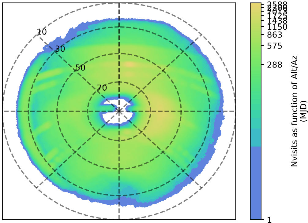
roll_pause_mjdp180_v3.4_10yrs r: Nvisits as function of Alt/Az
