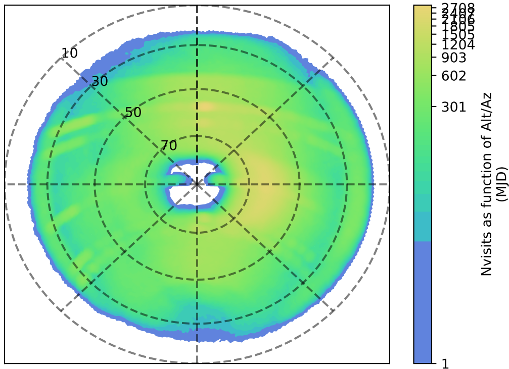
roll_pause_mjdp180_v3.4_10yrs i: Nvisits as function of Alt/Az
