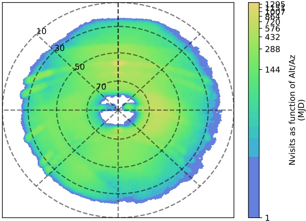
roll_pause_mjdp180_v3.4_10yrs g: Nvisits as function of Alt/Az
