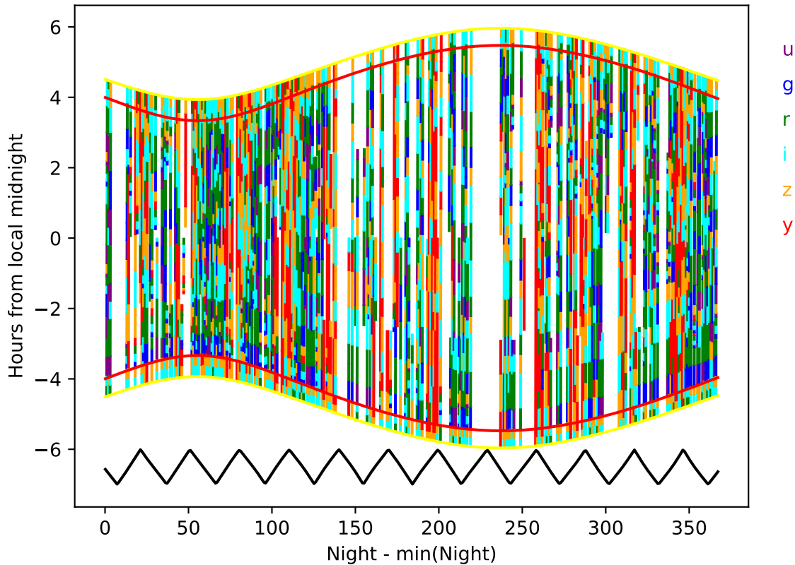
roll_pause_mjdp180_v3.4_10yrs year 7-8: Hourglass
