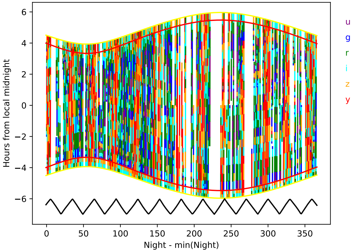
roll_pause_mjdp180_v3.4_10yrs year 3-4: Hourglass
