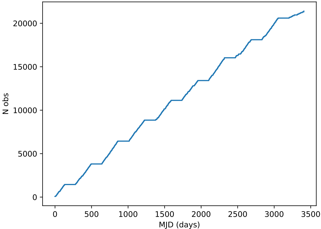
roll_pause_mjdp180_v3.4_10yrs note like DD:ECDFS%: Cumulative
