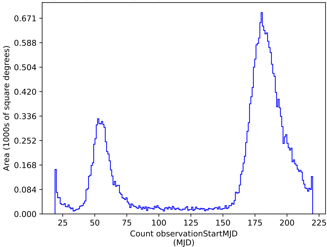
roll_pause_mjdp180_v3.4_10yrs r: Count observationStartMJD
