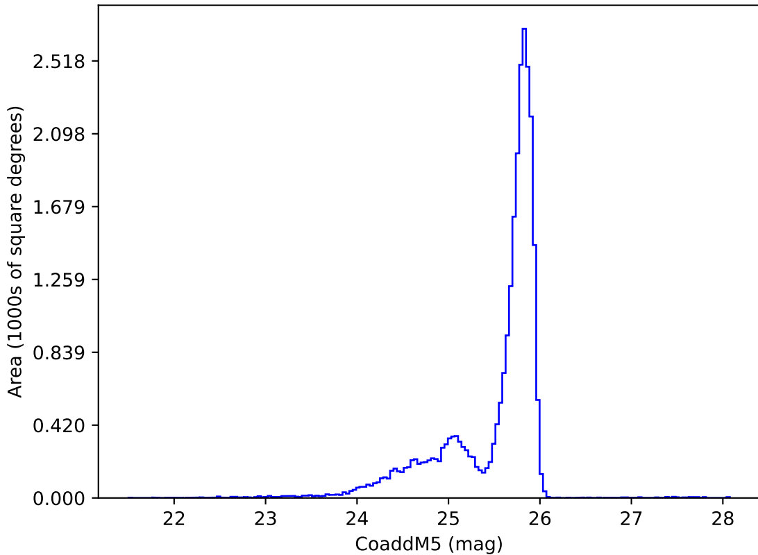
roll_pause_mjdp180_v3.4_10yrs z: CoaddM5
