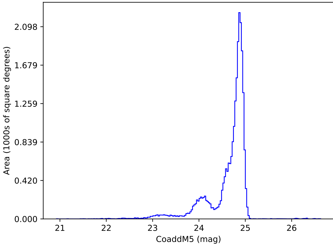
roll_pause_mjdp180_v3.4_10yrs y: CoaddM5
