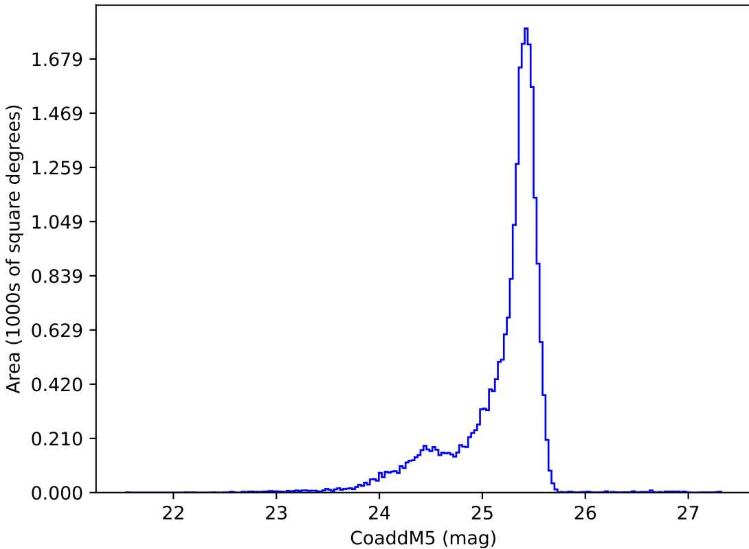
roll_pause_mjdp180_v3.4_10yrs u: CoaddM5
