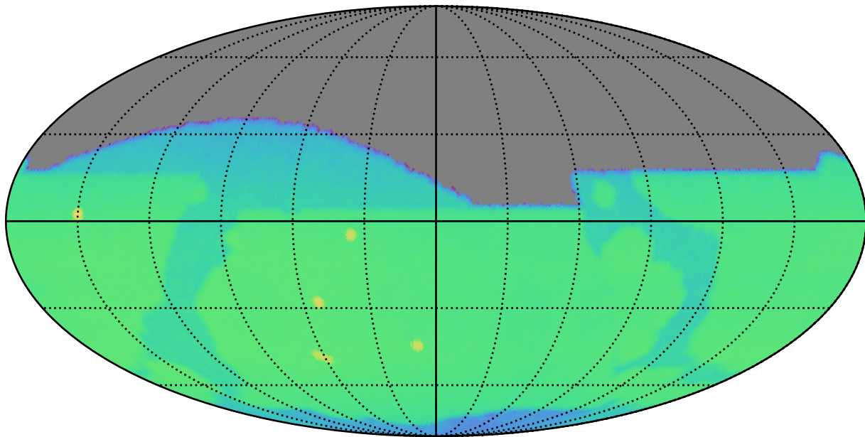
roll_pause_mjdp180_v3.4_10yrs r: CoaddM5
