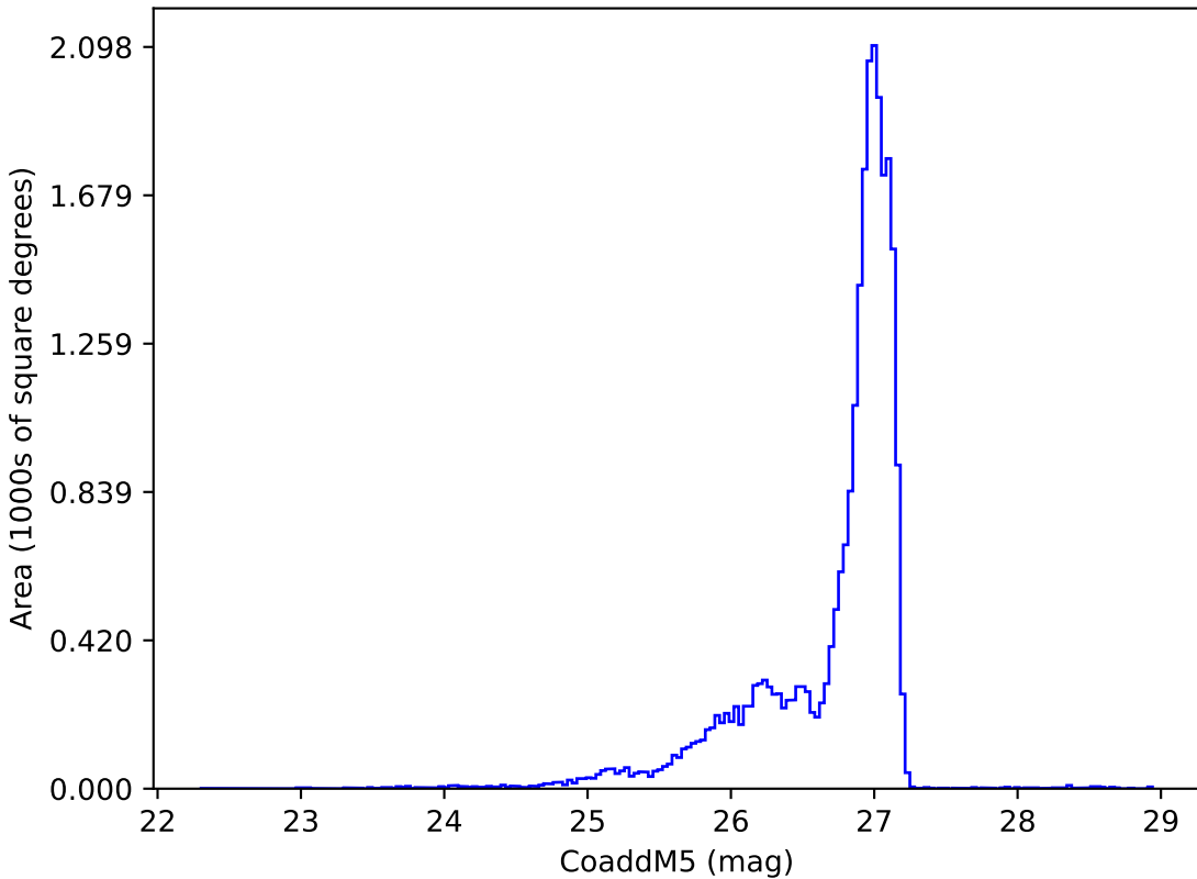
roll_pause_mjdp180_v3.4_10yrs r: CoaddM5
