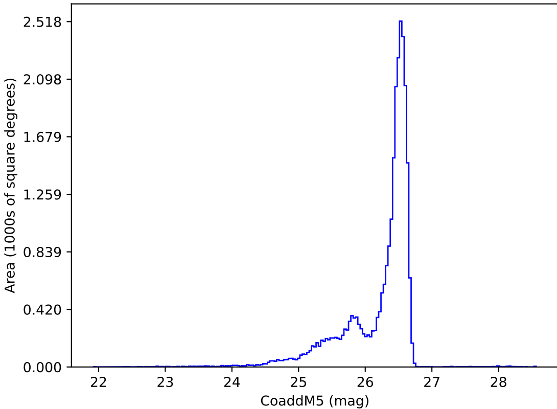
roll_pause_mjdp180_v3.4_10yrs i: CoaddM5
