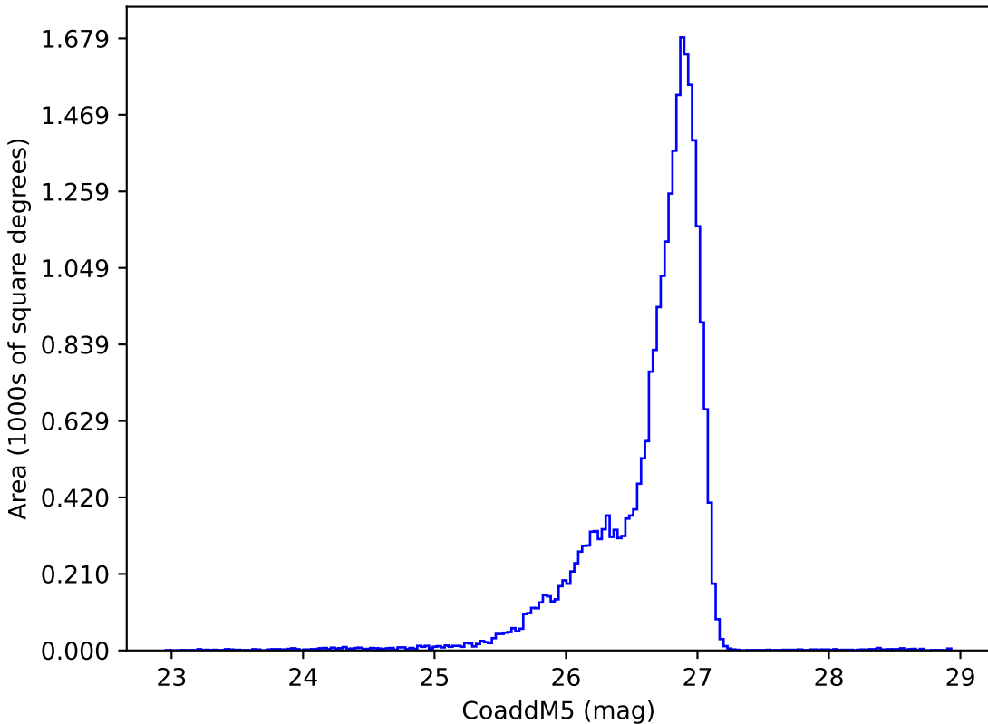
roll_pause_mjdp180_v3.4_10yrs g: CoaddM5
