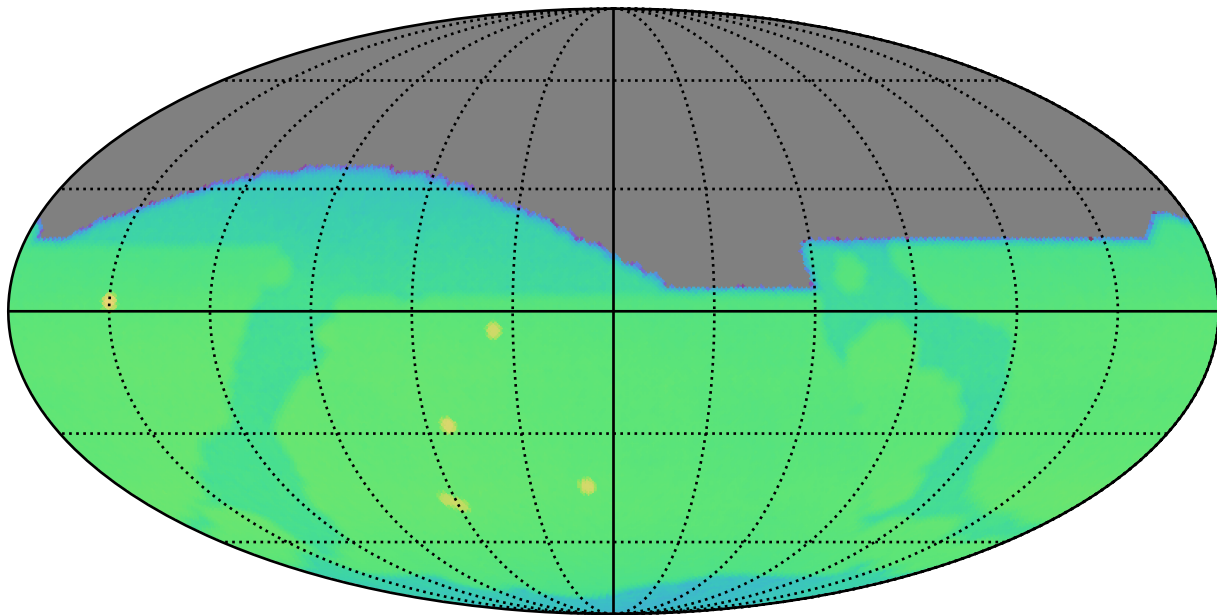
roll_pause_mjdp180_v3.4_10yrs : CoaddM5
