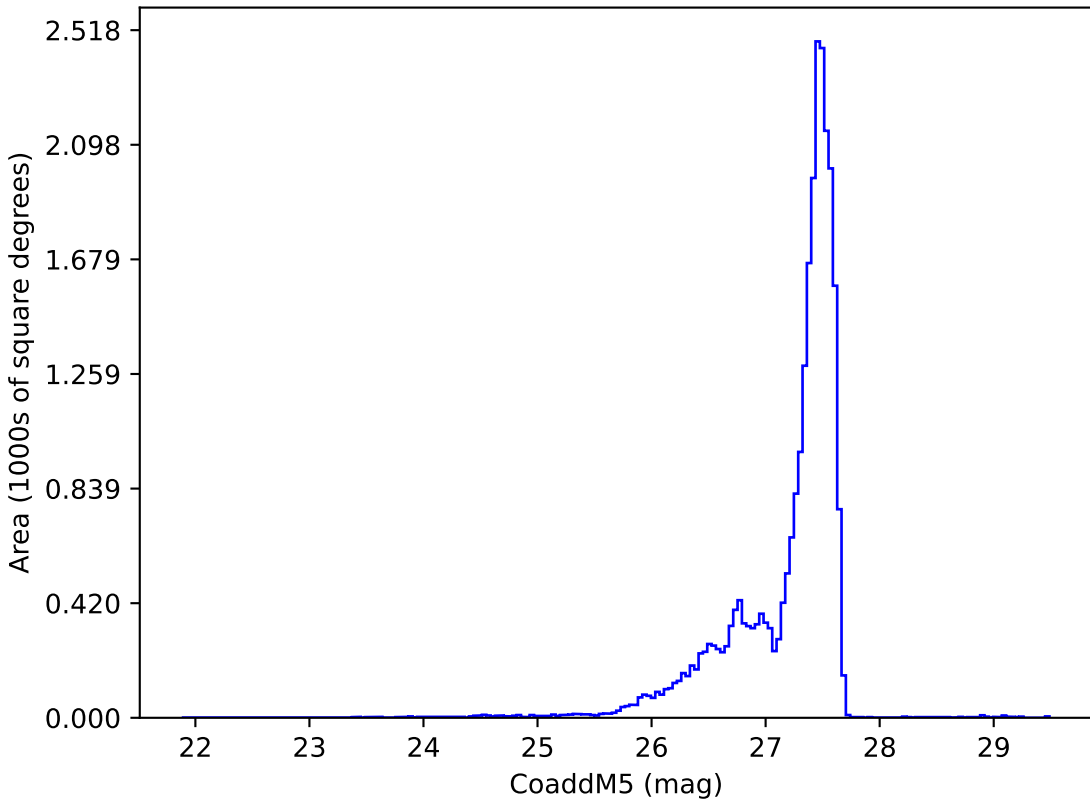
roll_pause_mjdp180_v3.4_10yrs : CoaddM5
