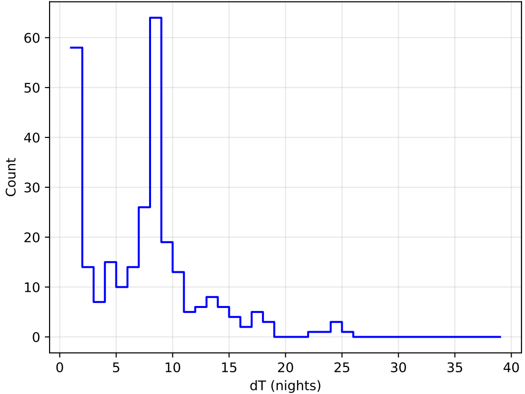
roll_pause_mjdp180_v3.4_10yrs all bands: DD:XMM_LSS Delta Nights Histogram
